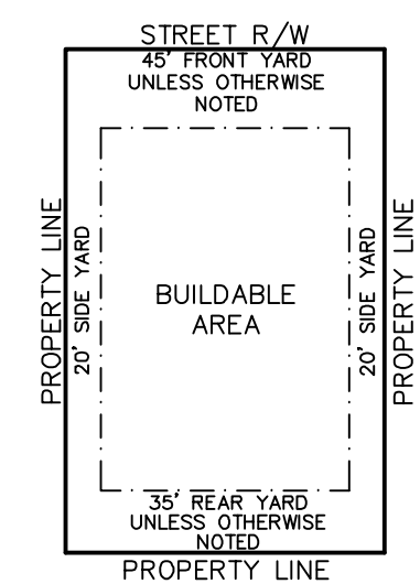
TYPICAL SUBDIVISION LOT (RS-3 ZONING)
