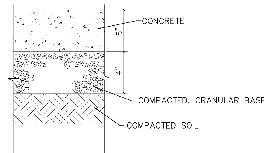
CONCRETE SIDEWALK
