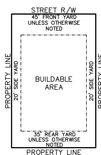
TYPICAL SUBDIVISION LOT (RS-3 ZONING)
