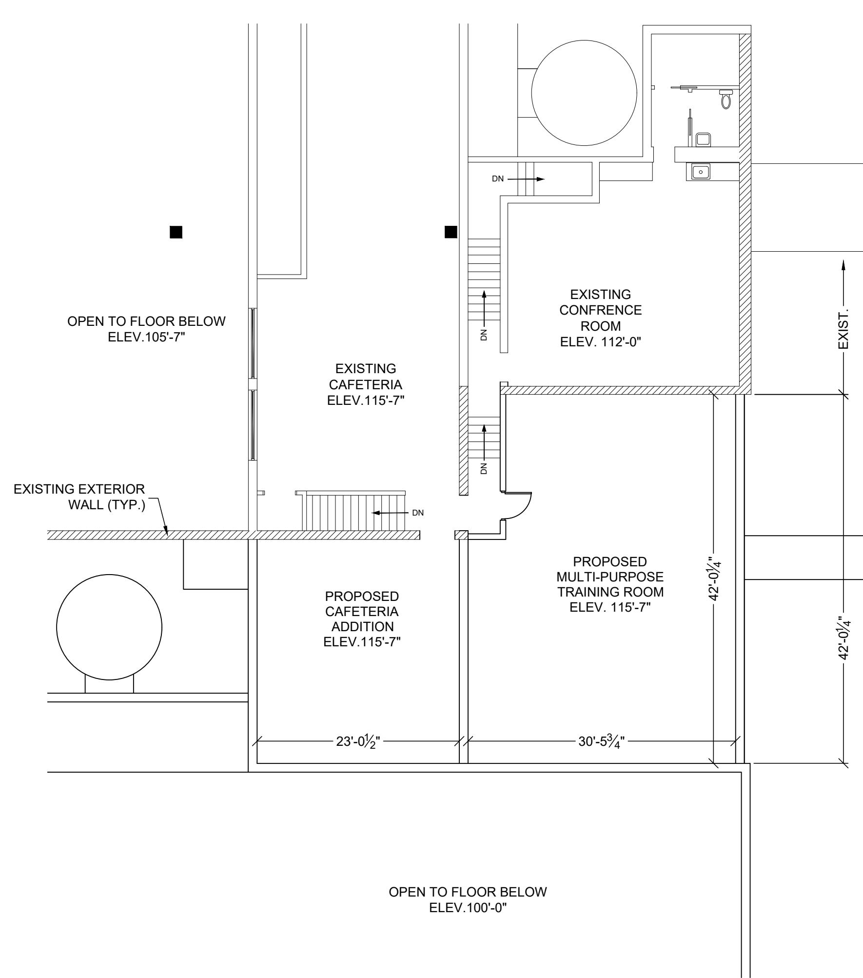
SECOND FLOOR PLAN SCALE: 3/32" = 1'-0"
